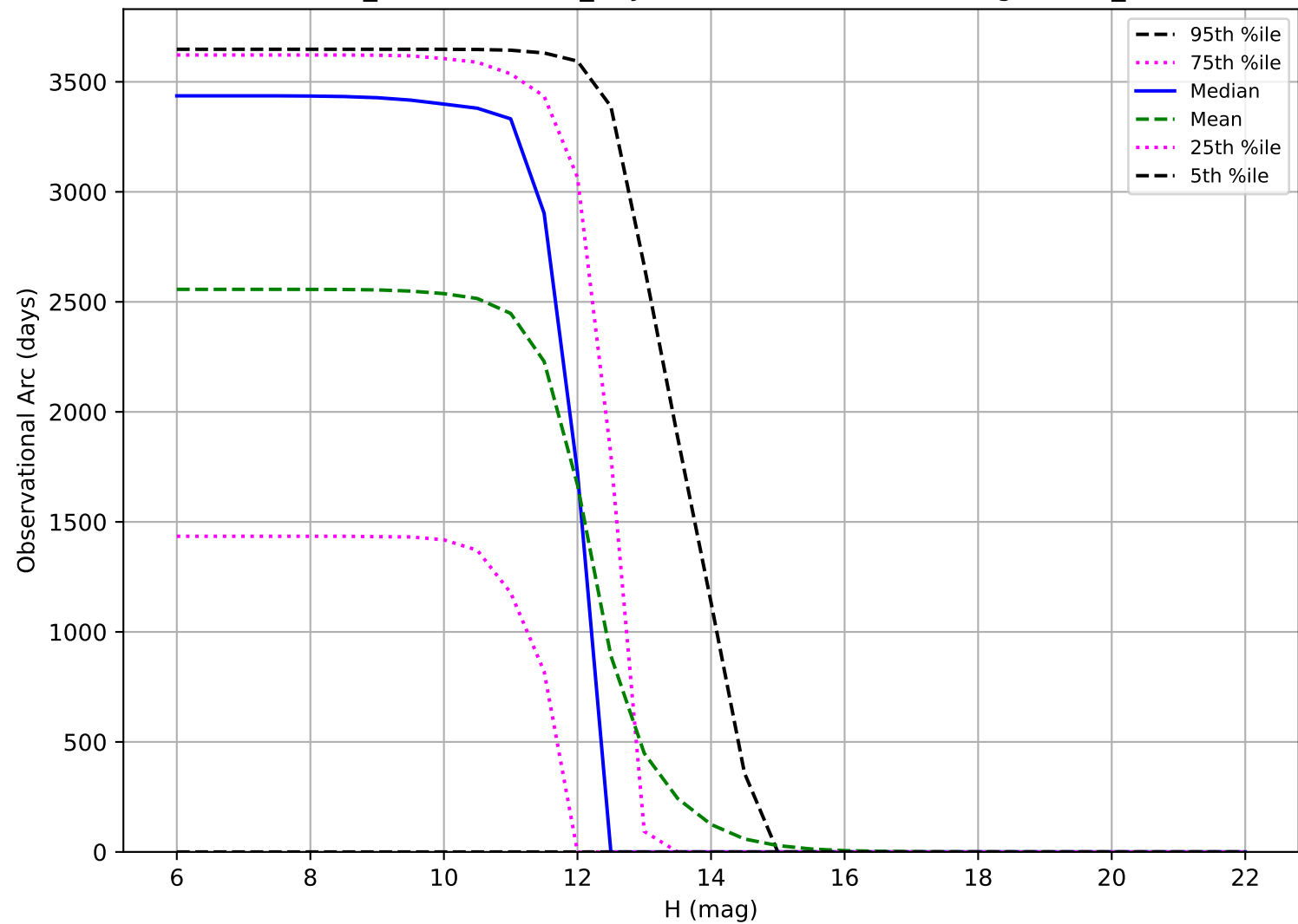
weather_cloudso14v3.5_10yrs: Observational Arc Length OCC_r20
