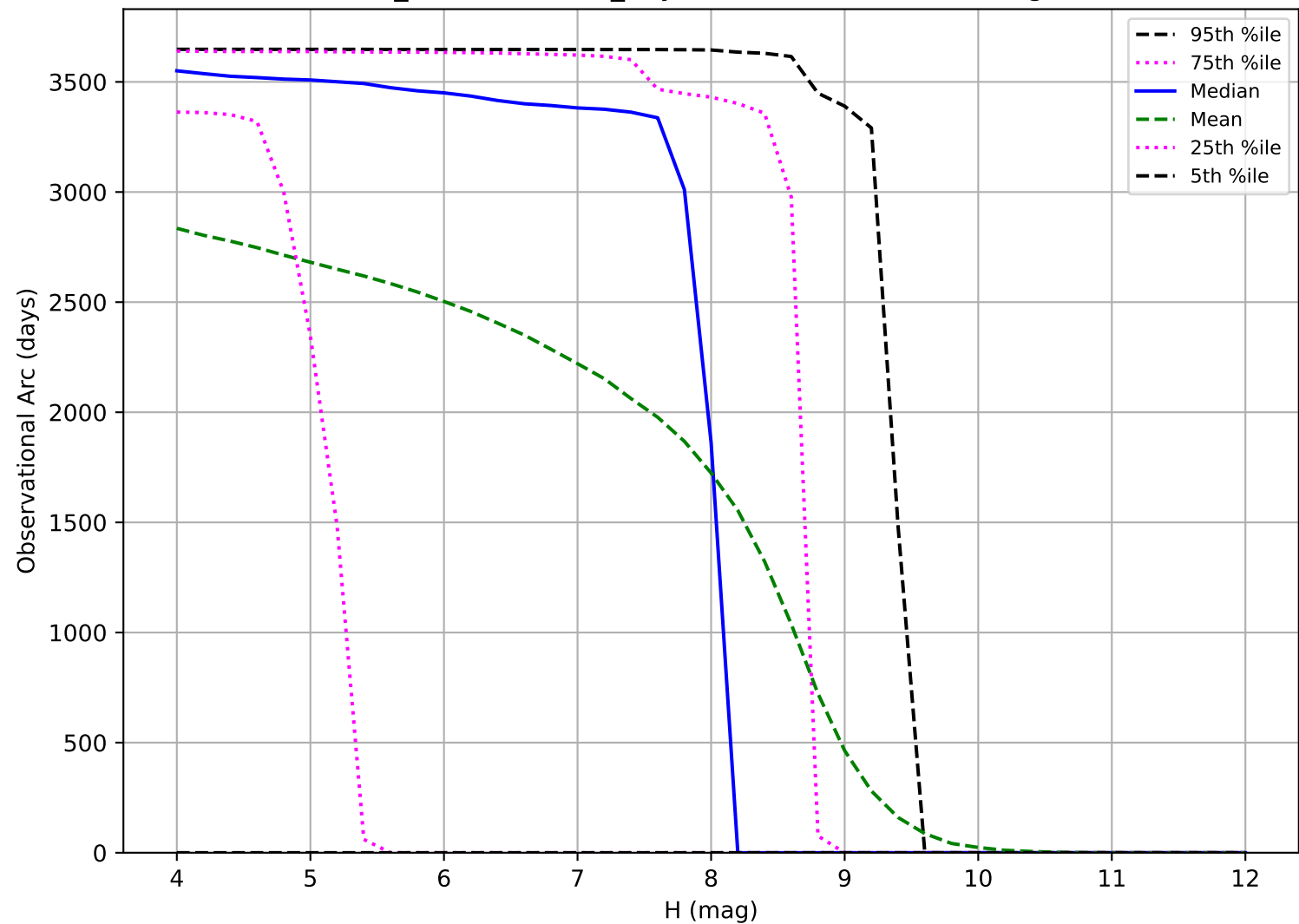
weather_cloudso14v3.5_10yrs: Observational Arc Length TNO
