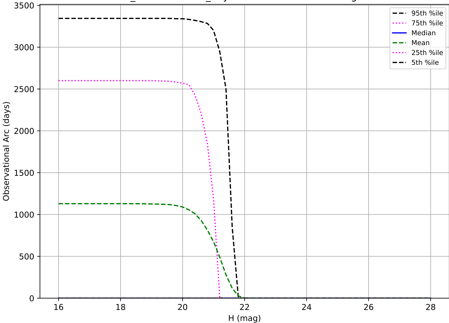
weather_cloudso14v3.5_10yrs: Observational Arc Length Vatra
