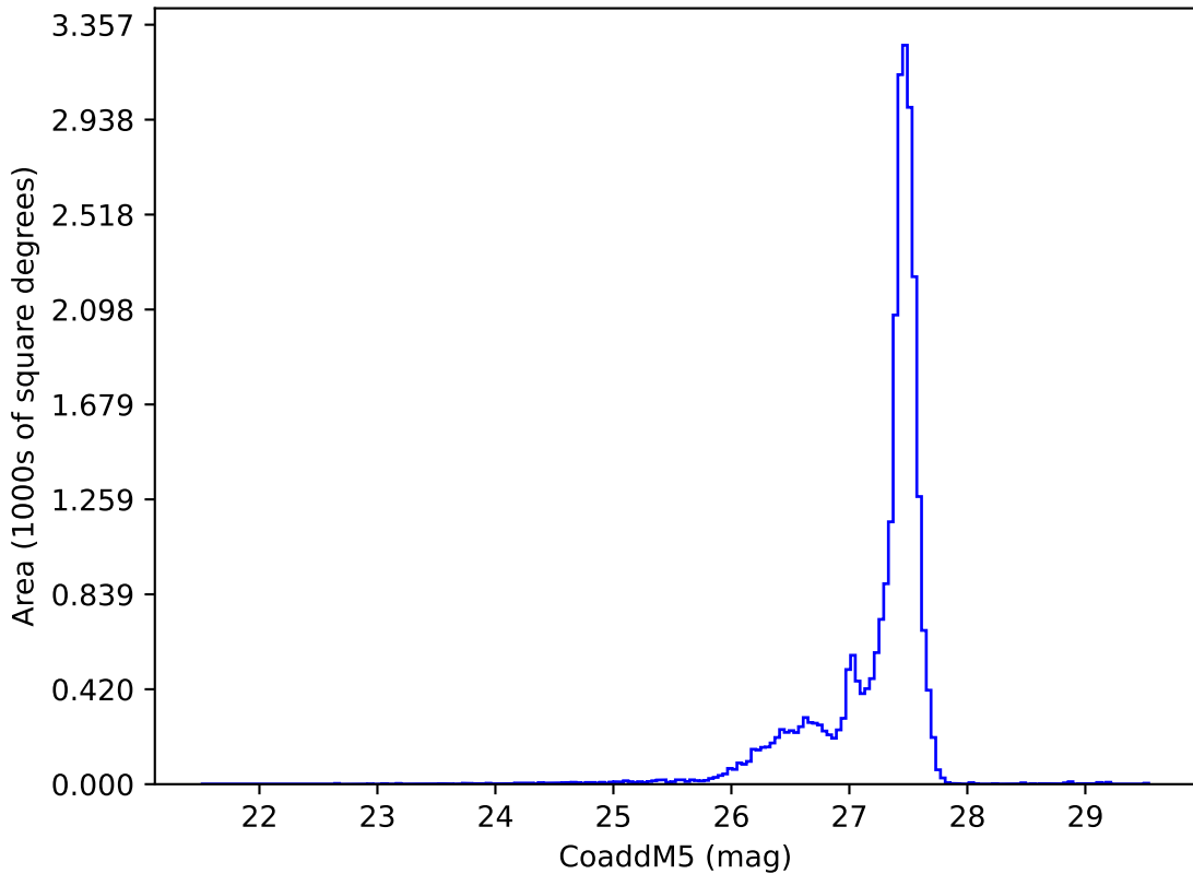
weather_cloudso16v3.5_10yrs : CoaddM5
