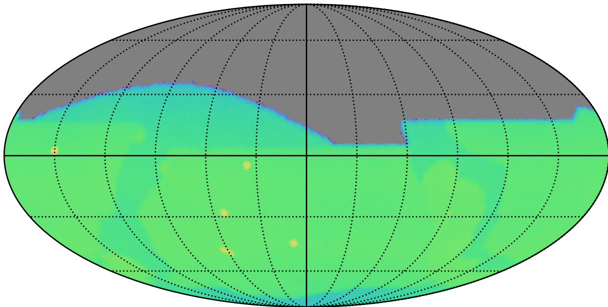
weather_cloudso16v3.5_10yrs : CoaddM5
