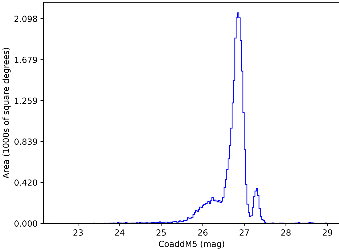
weather_cloudso16v3.5_10yrs g: CoaddM5
