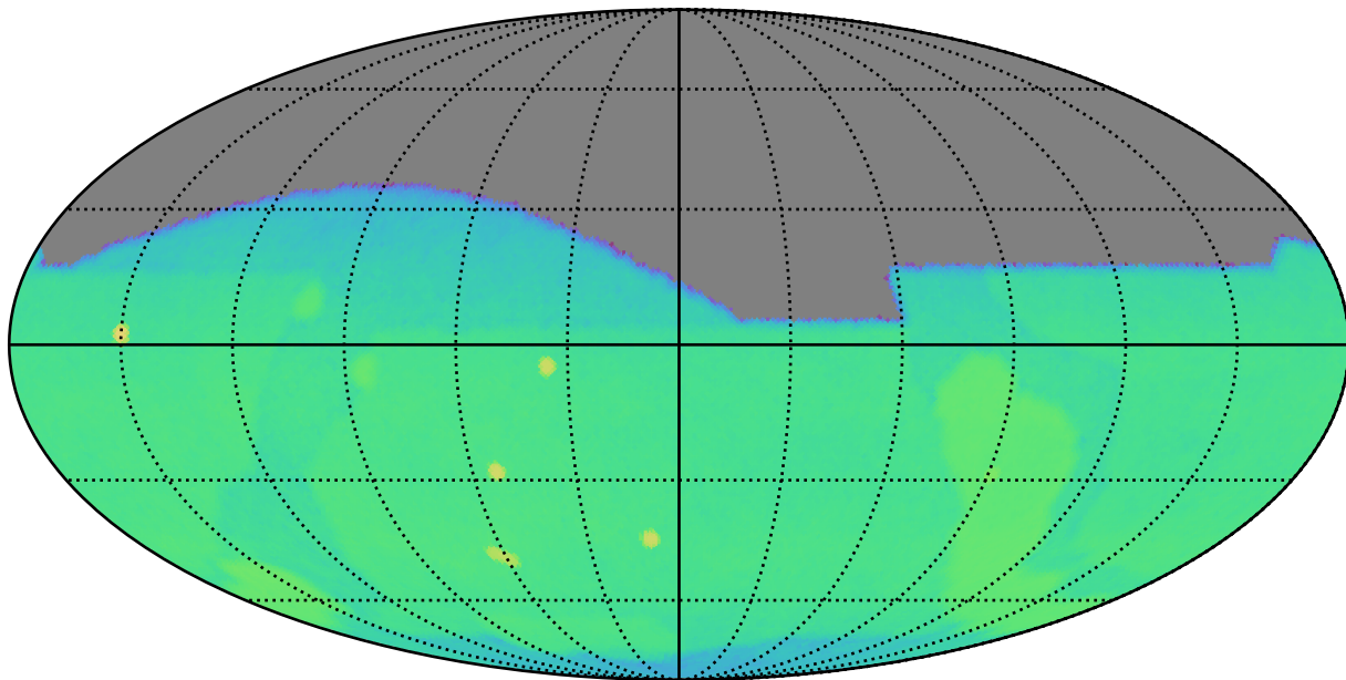
weather_cloudso16v3.5_10yrs g: CoaddM5
