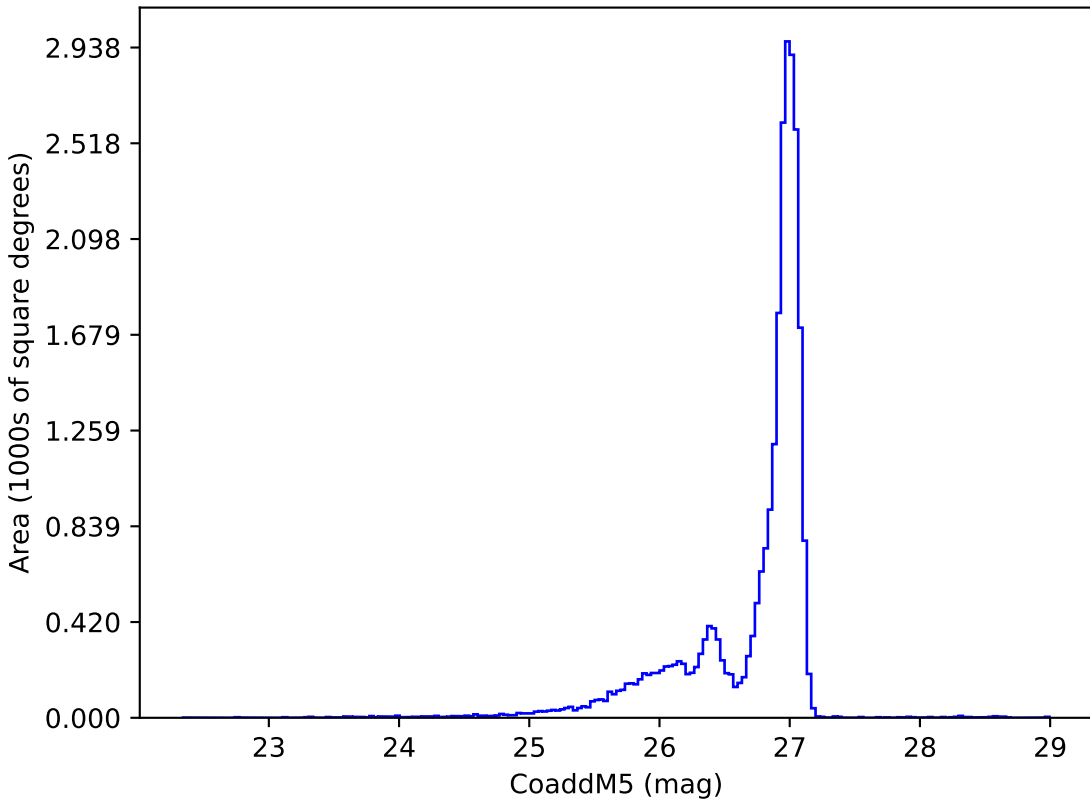
weather_cloudso16v3.5_10yrs r: CoaddM5
