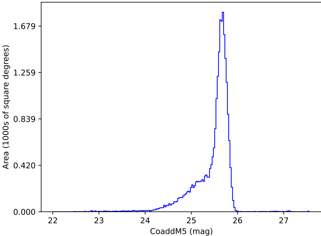
weather_cloudso16v3.5_10yrs u: CoaddM5
