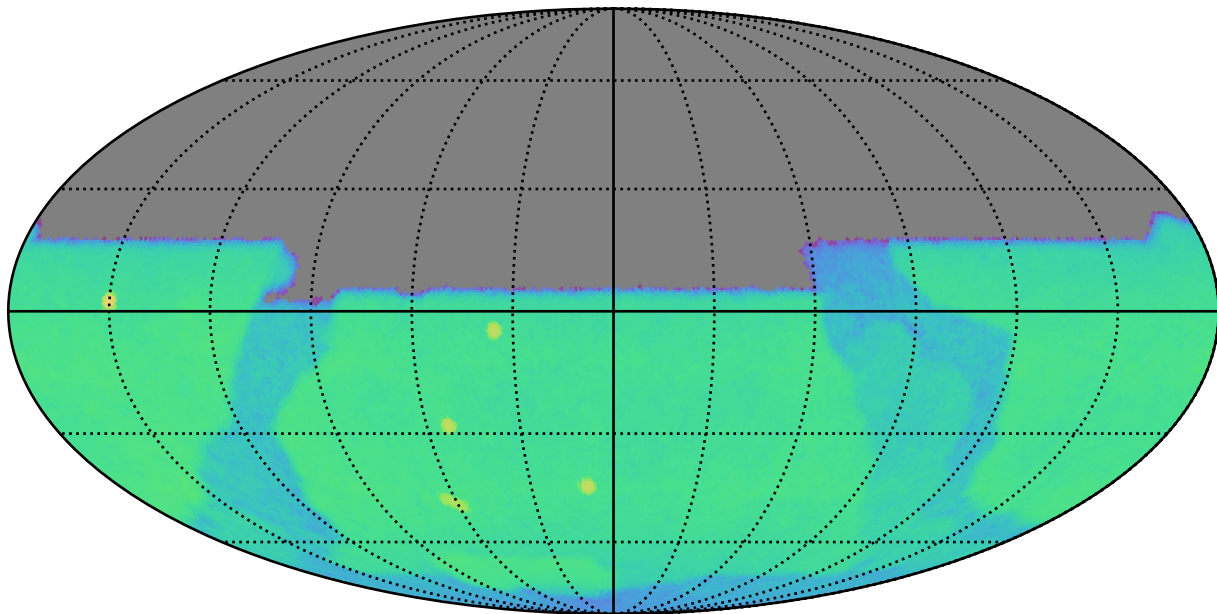
weather_cloudso16v3.5_10yrs u: CoaddM5
