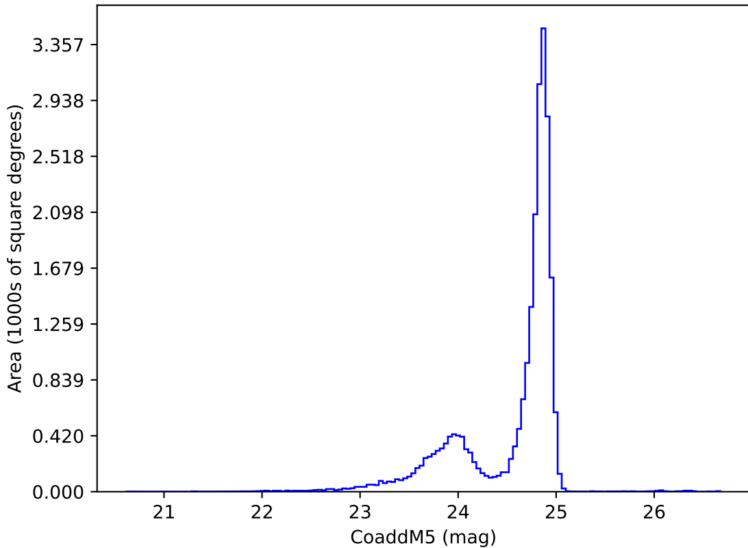
weather_cloudso16v3.5_10yrs y: CoaddM5
