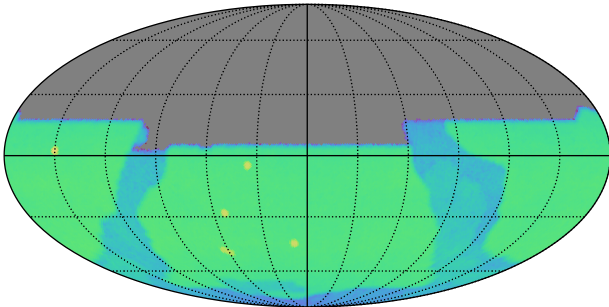
weather_cloudso16v3.5_10yrs y: CoaddM5
