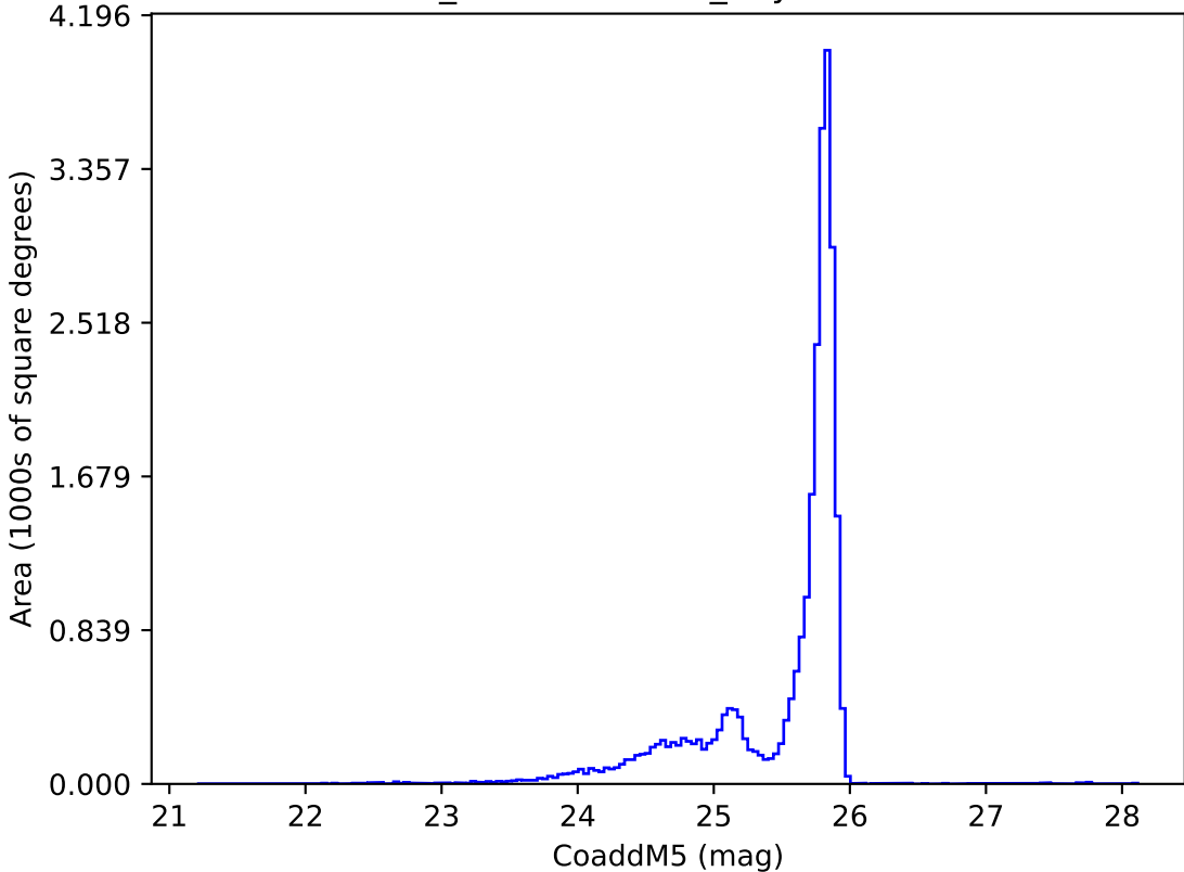
weather_cloudso16v3.5_10yrs z: CoaddM5
