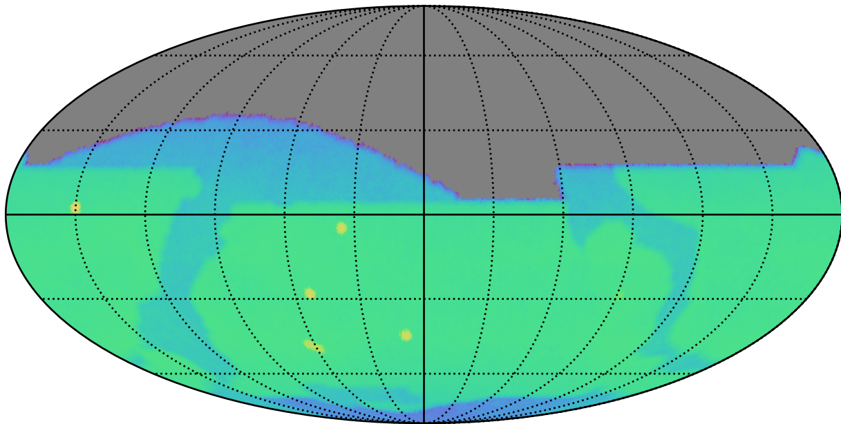
weather_cloudso16v3.5_10yrs z: CoaddM5
