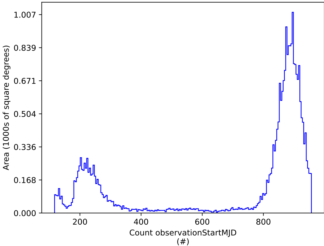
weather_cloudso16v3.5_10yrs : Count observationStartMJD
