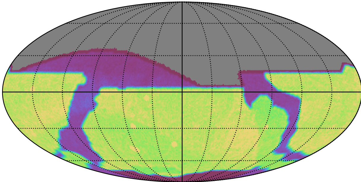
weather_cloudso16v3.5_10yrs : Count observationStartMJD
