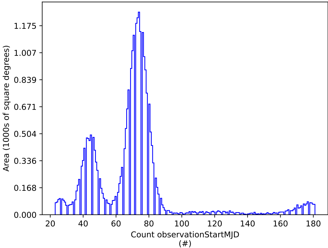
weather_cloudso16v3.5_10yrs g: Count observationStartMJD
