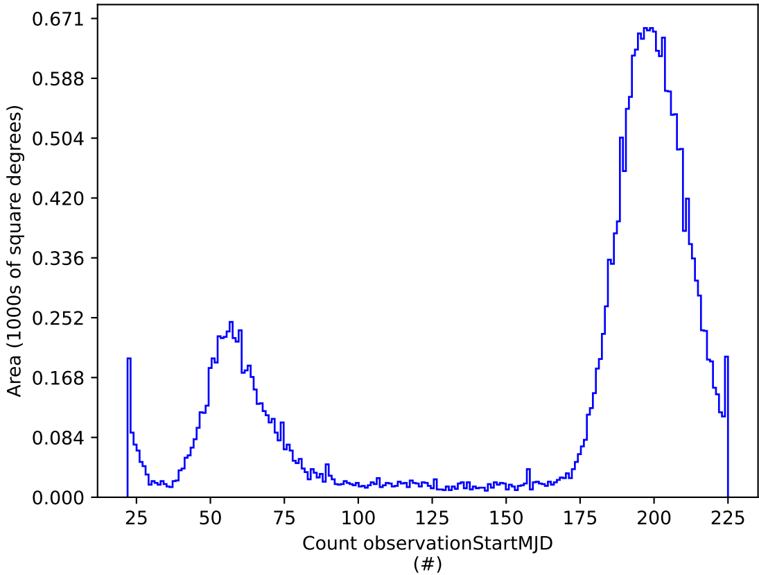
weather_cloudso16v3.5_10yrs i: Count observationStartMJD
