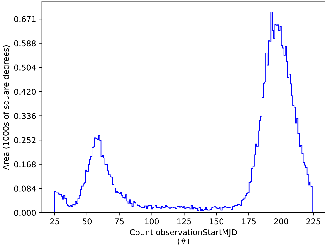
weather_cloudso16v3.5_10yrs r: Count observationStartMJD
