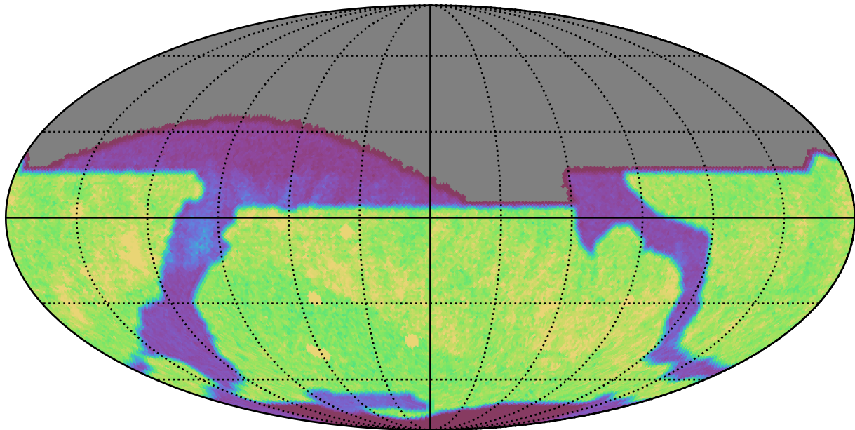
weather_cloudso16v3.5_10yrs z: Count observationStartMJD
