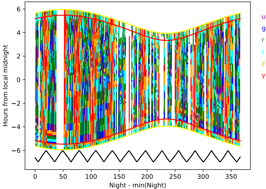
weather_cloudso16v3.5_10yrs year 2-3: Hourglass
