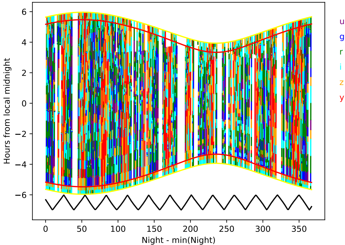
weather_cloudso16v3.5_10yrs year 7-8: Hourglass
