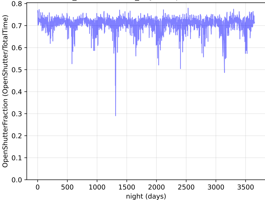
weather_cloudso16v3.5_10yrs : OpenShutterFraction
