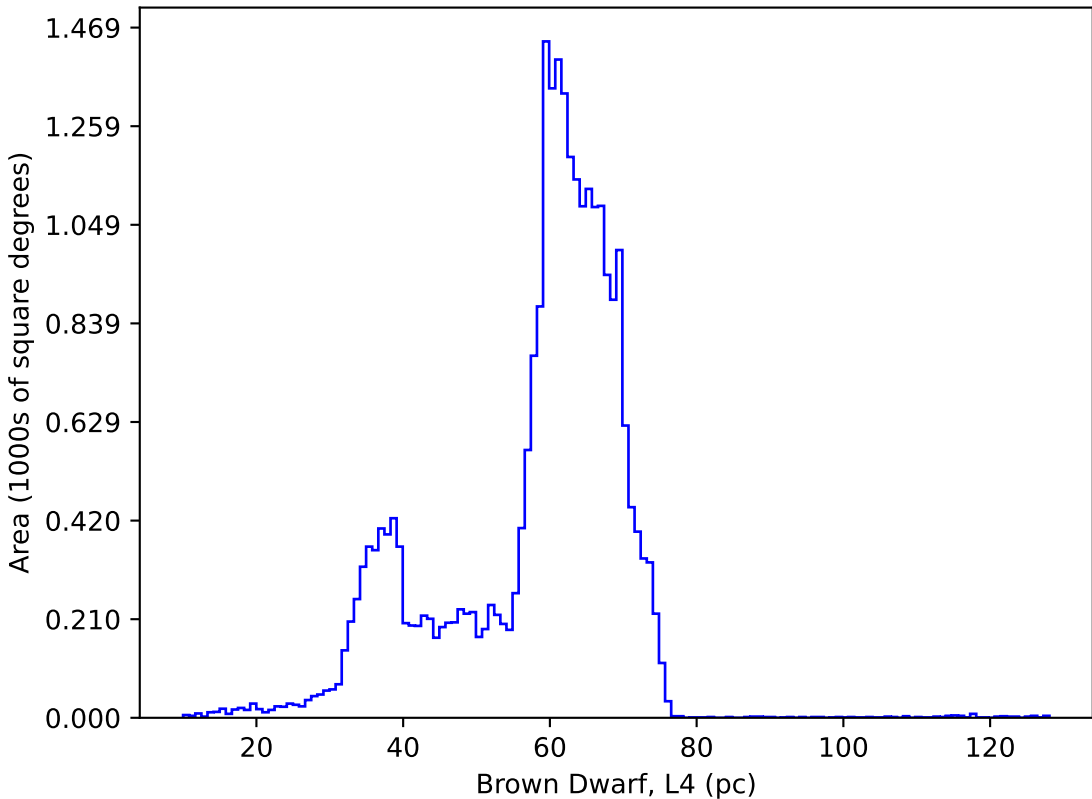
weather_cloudso16v3.5_10yrs : Brown Dwarf, L4
