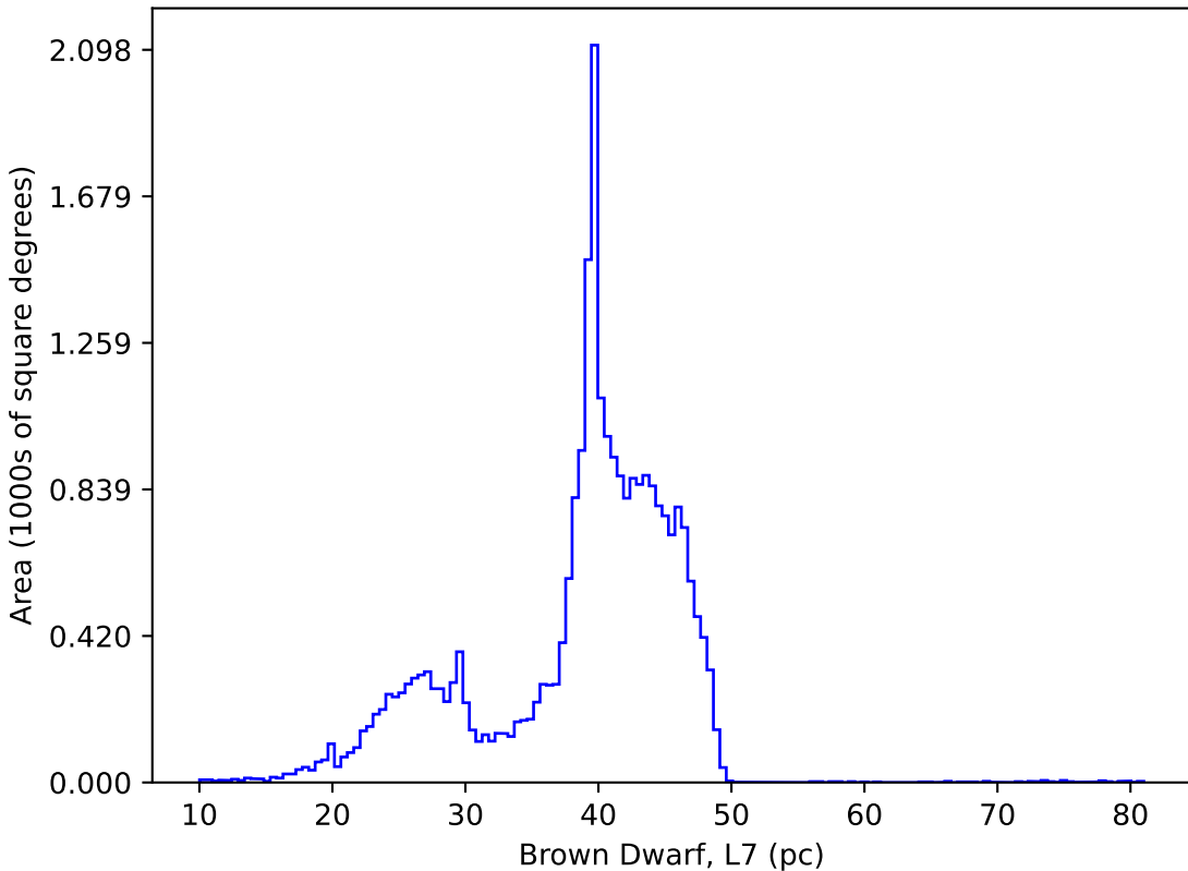
weather_cloudso16v3.5_10yrs : Brown Dwarf, L7
