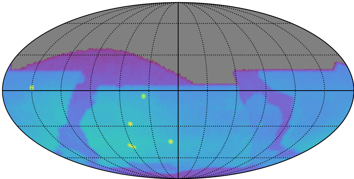
weather_cloudso16v3.5_10yrs : Brown Dwarf, L7
