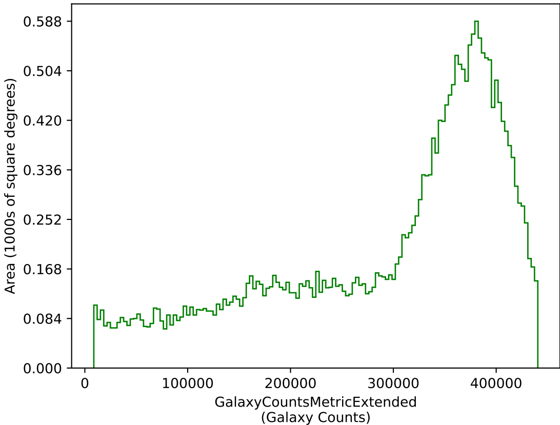
weather_cloudso16v3.5_10yrs g: GalaxyCountsMetricExtended
