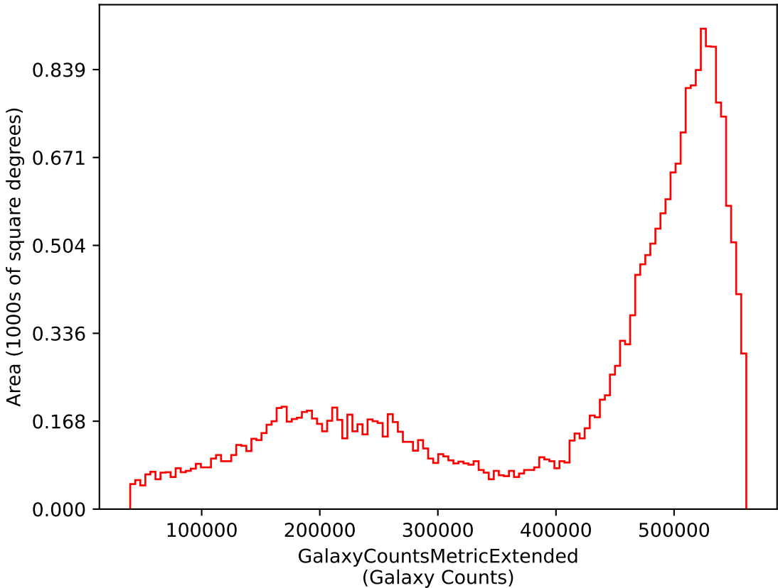
weather_cloudso16v3.5_10yrs i: GalaxyCountsMetricExtended
