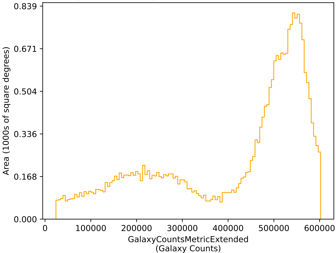
weather_cloudso16v3.5_10yrs r: GalaxyCountsMetricExtended
