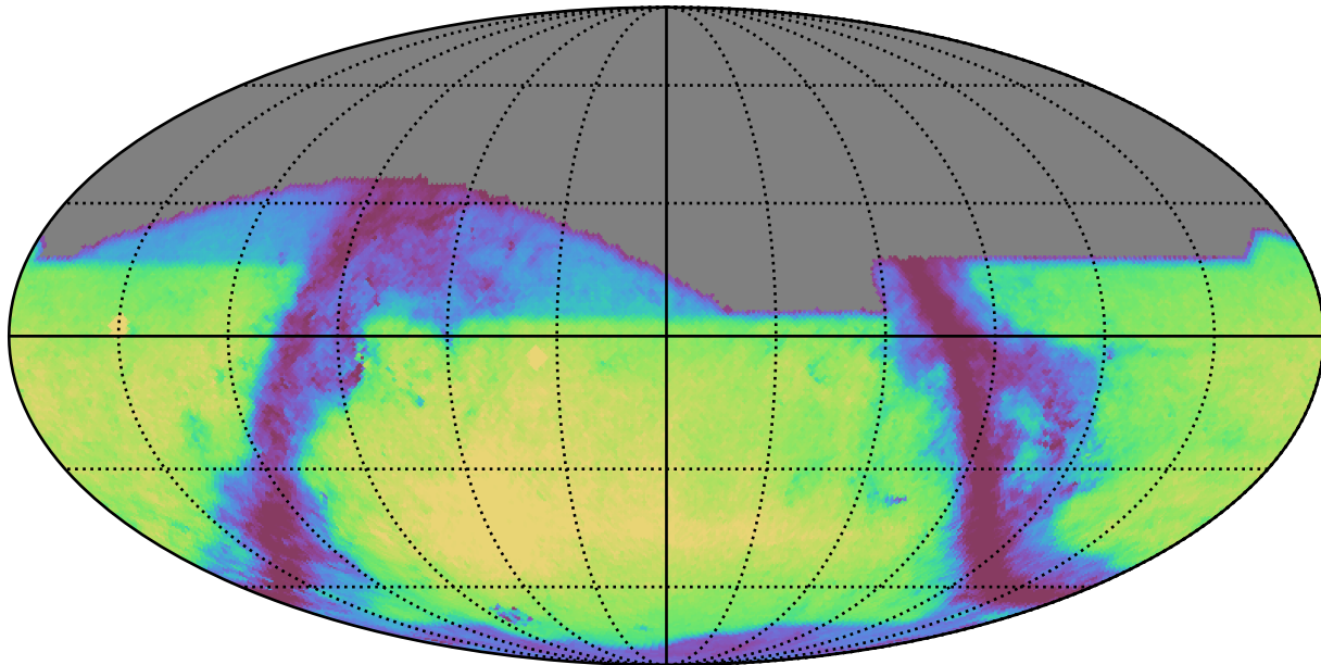
weather_cloudso16v3.5_10yrs r: GalaxyCountsMetricExtended
