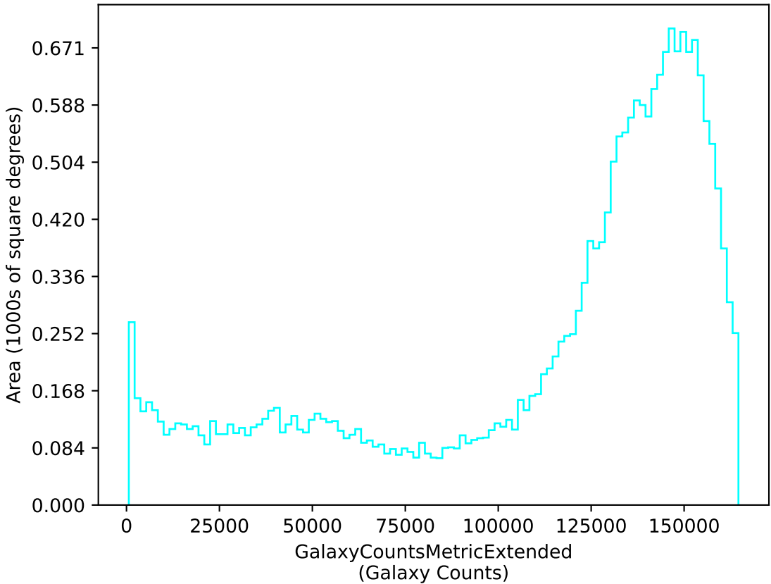
weather_cloudso16v3.5_10yrs u: GalaxyCountsMetricExtended
