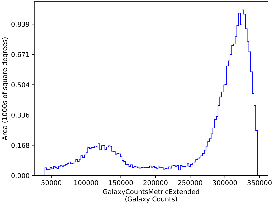
weather_cloudso16v3.5_10yrs y: GalaxyCountsMetricExtended
