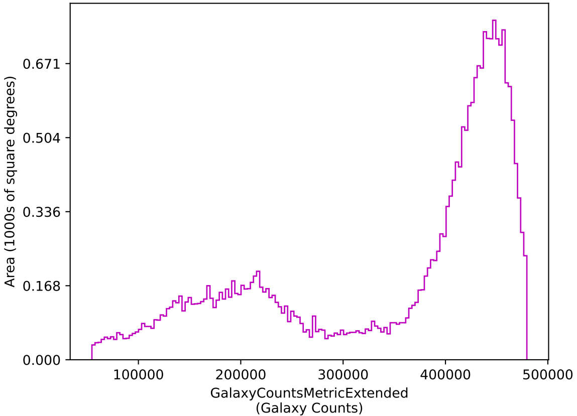
weather_cloudso16v3.5_10yrs z: GalaxyCountsMetricExtended
