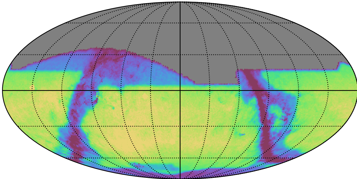
weather_cloudso16v3.5_10yrs z: GalaxyCountsMetricExtended
