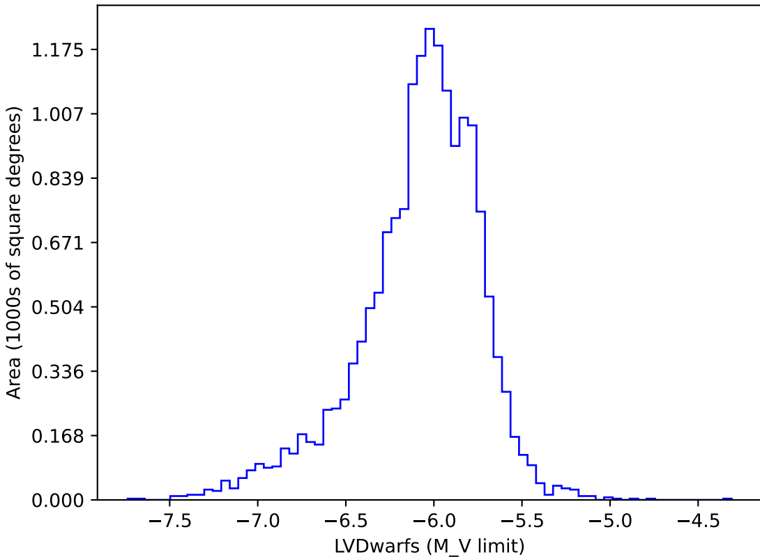
weather_cloudso16v3.5_10yrs gi: LVDwarfs
