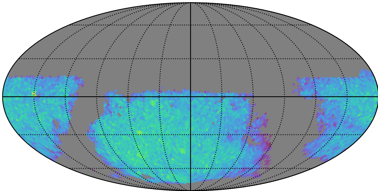
weather_cloudso16v3.5_10yrs gi: LVDwarfs
