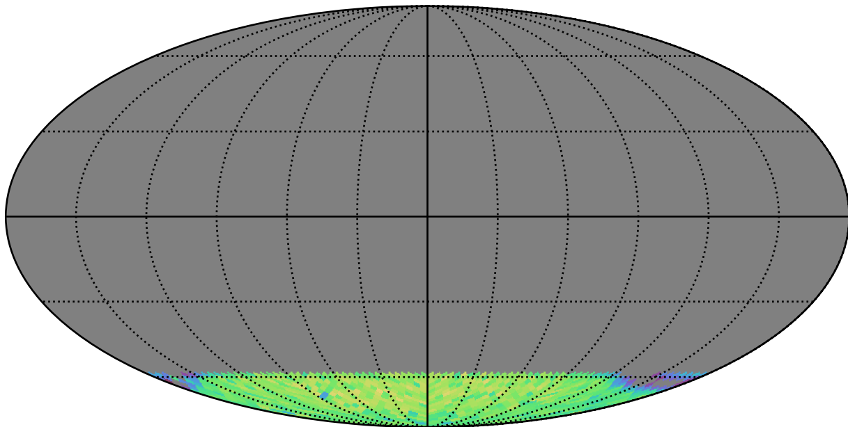
weather_cloudso16v3.5_10yrs gi SCP: LVDwarfs
