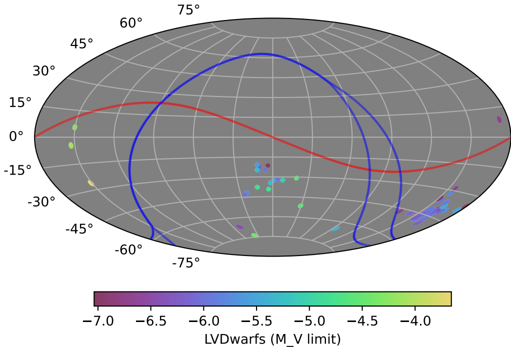
weather_cloudso16v3.5_10yrs gi: LVDwarfs
