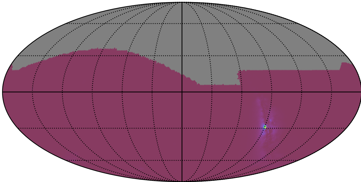
weather_cloudso16v3.5_10yrs : NlcPoints
