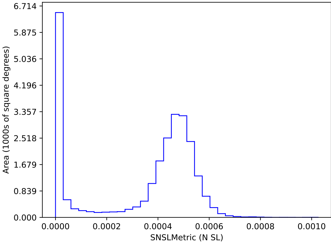
weather_cloudso16v3.5_10yrs : SNSLMetric
