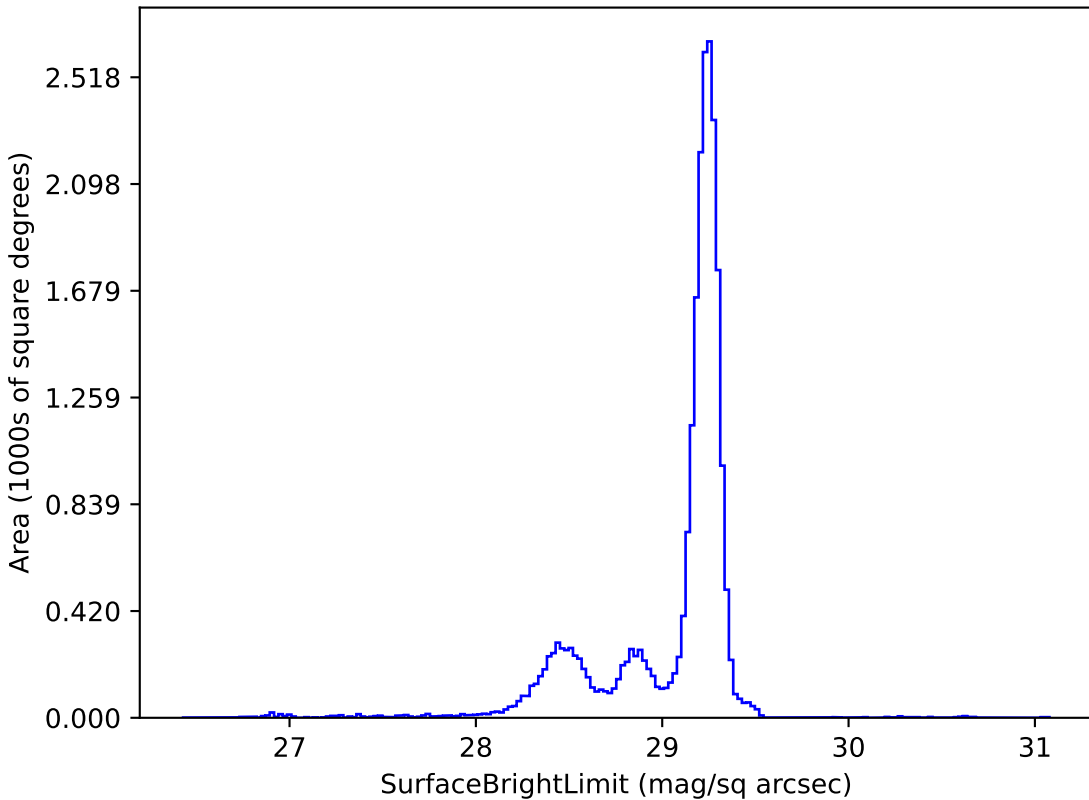
weather_cloudso16v3.5_10yrs u: SurfaceBrightLimit
