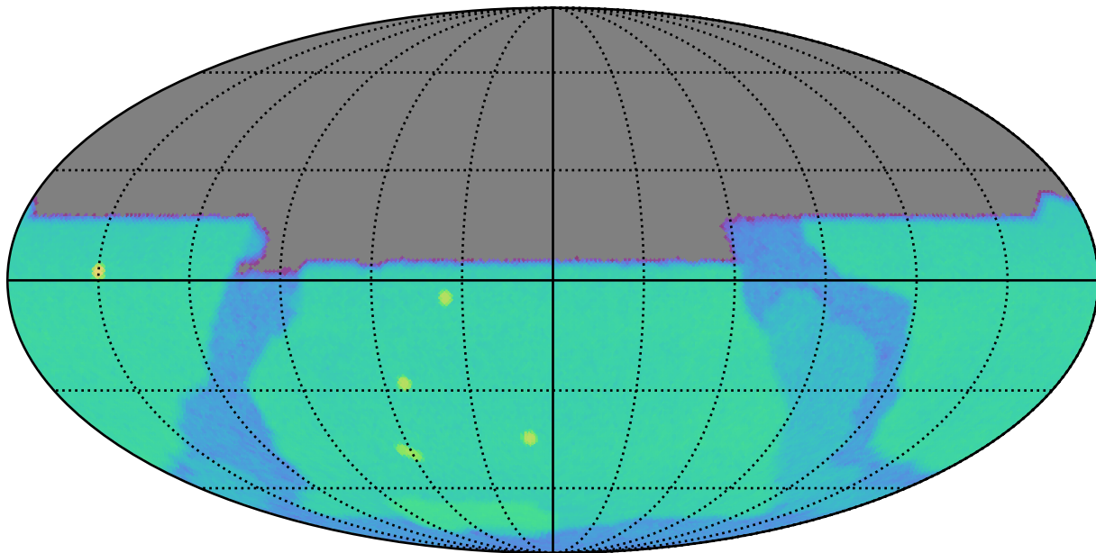
weather_cloudso16v3.5_10yrs u: SurfaceBrightLimit
