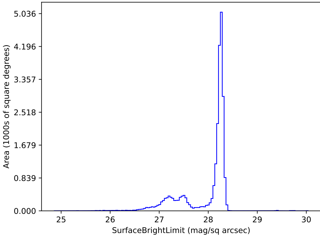
weather_cloudso16v3.5_10yrs y: SurfaceBrightLimit
