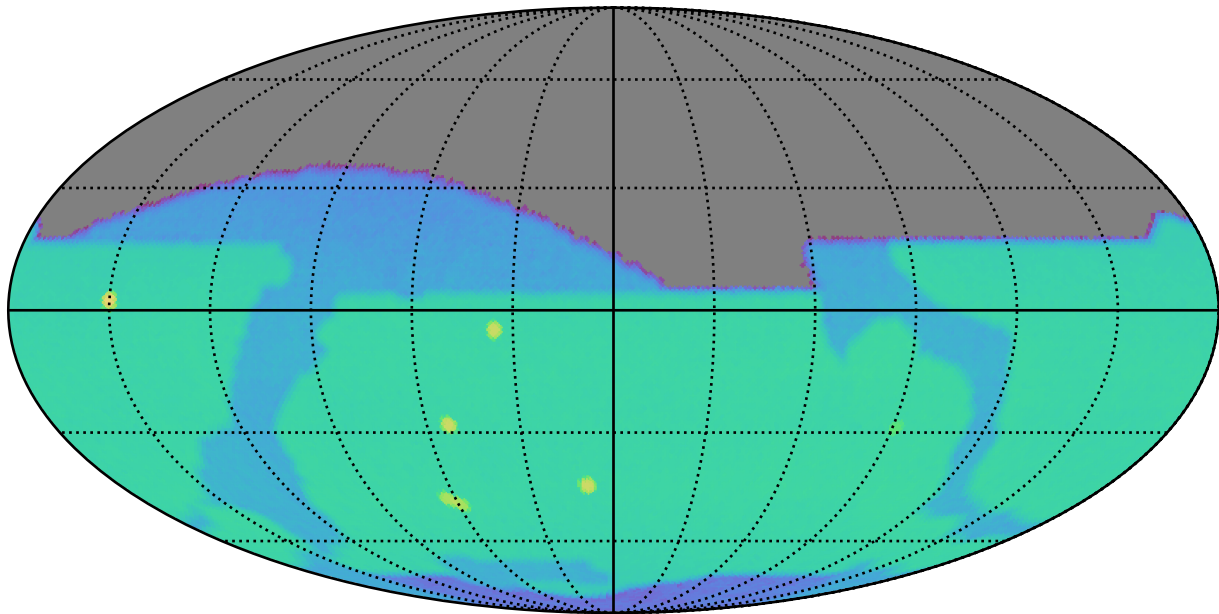
weather_cloudso16v3.5_10yrs z: SurfaceBrightLimit
