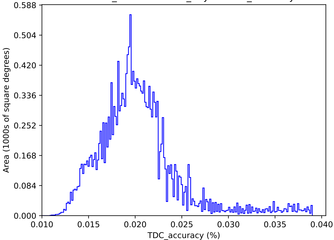
weather_cloudso16v3.5_10yrs : TDC_accuracy
