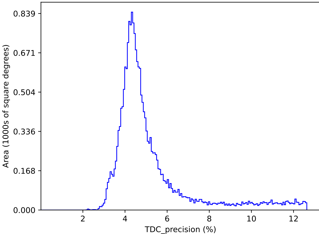
weather_cloudso16v3.5_10yrs : TDC_precision
