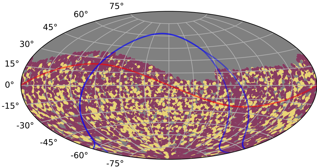
weather_cloudso16v3.5_10yrs : TDEsPopMetric_prepeak
