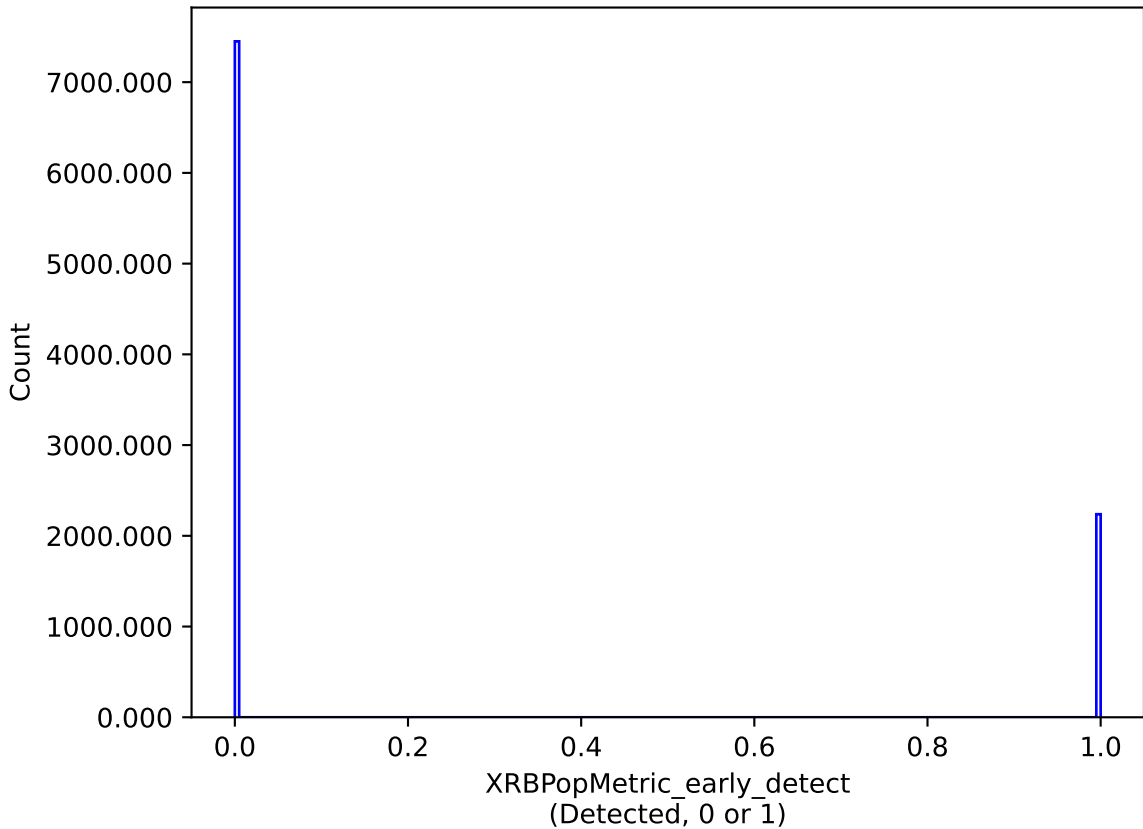
weather_cloudso16v3.5_10yrs : XRBPoMetric_early_detect
