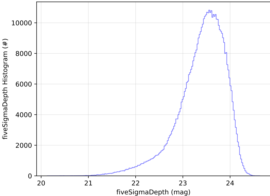
weather_cloudso16v3.5_10yrs i: fiveSigmaDepth Histogram
