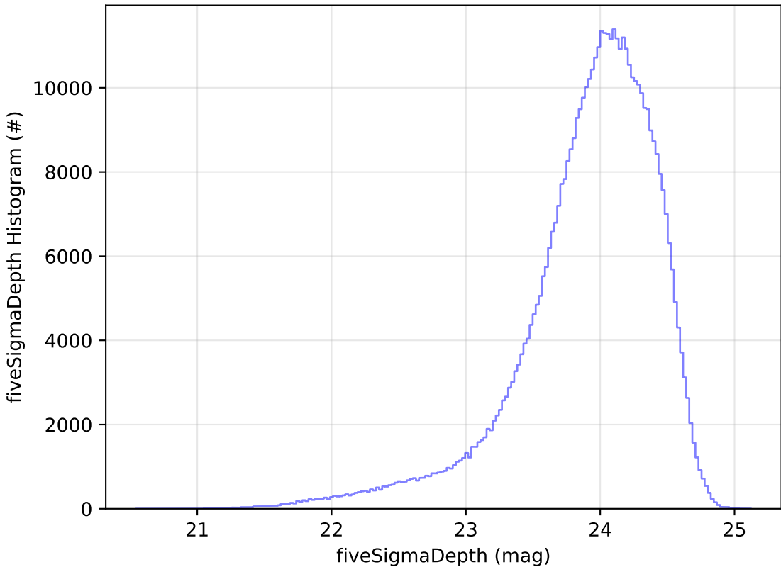
weather_cloudso16v3.5_10yrs r: fiveSigmaDepth Histogram
